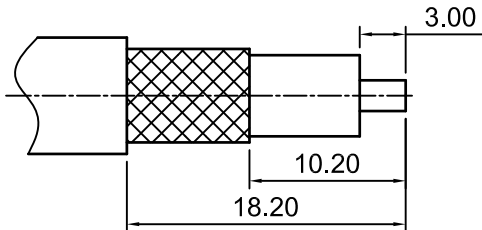
RECOMMENDED STRIPPING DIMENSION
