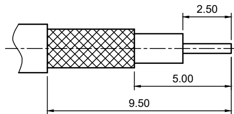
RECOMMENDED STRIP DIMENSION
