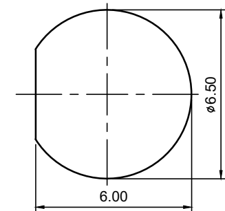
RECOMMENDED MOUNT HOLE
